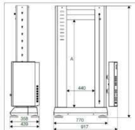
Principle drawing of the ProLine ZD05/ZD20 TM
